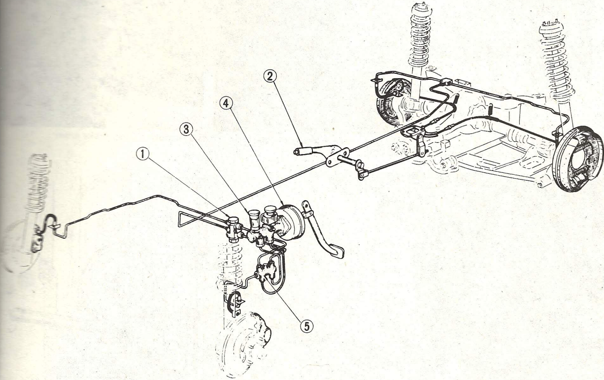
Fig. 9.2. Braking system - 260Z models
