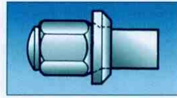
Ford Ghia open nuts – zinc plated 12mm 1.5 Sleeve nut with 60° Ghia washer
